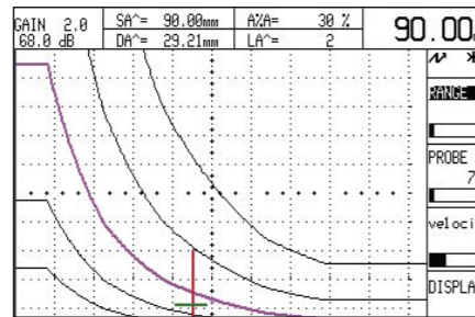
DAC Curve with 6 dB offset multiple curves
