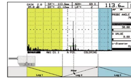
New "Color Leg" indicator displays the legs of the angle beam inspection in different colors
